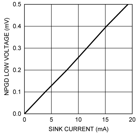
Figure 6. nPGD Low Voltage (PGD VOL ) vs Sink Current
